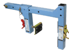
ADJUSTABLE PARAPET WALL ANCHOR No tools required with simple clamp- on non-penetrating installation. Adjusts to fit parapets from 1/2" to 15" thick and having a minimum height of 9"
